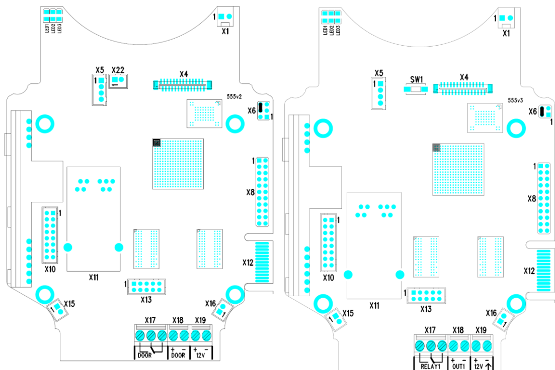
Figure 2.11 2N ® Helios IP Safety Connectors, PCB Version 555v2 and 555v3
